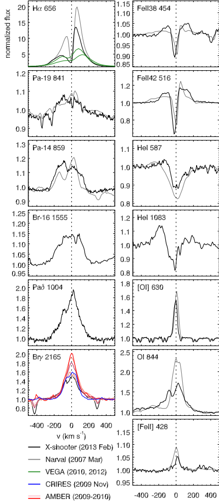
Figure 3. Selection of spectral lines of HD 50138 obtained with X-shooter, Narval (BF09), and AMBER. All lines show some degree of variability. Note the varying strength of double peaks and the component at v \sim 0 \text{ km s}^{-1} . The Narval and CRIFES spectra are rebinned to match the X-shooter resolution (9100 in the optical, 17,400 in the NIR).
