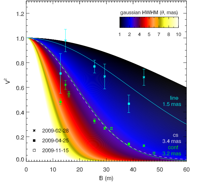
Figure 6. Average V_{\text{cont}}^2 , V_{\text{line}}^2 values plotted as a function of baseline. The colored surface corresponds to the V^2 of a grid of single-Gaussian models with half width at half maximum (HWHM) as indicated by the colors. The best-fit models are indicated for the continuum-emitting region (green solid line) and the \text{Br}\gamma line-emitting region ( \lambda_0 = 2166.167 \text{ nm} , cyan solid line). The fit to the stellar-flux-corrected continuum region ( V_{\text{cs}}^2 ) is also plotted (white dashed line).
