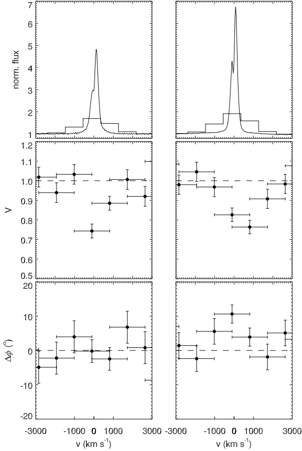
Figure 5. Top to bottom: H\alpha spectrum, squared visibility and differential phase taken with CHARA/VEGA, taken on 2010-10-11 (left panels) and 2012-10-29 (right panels).
