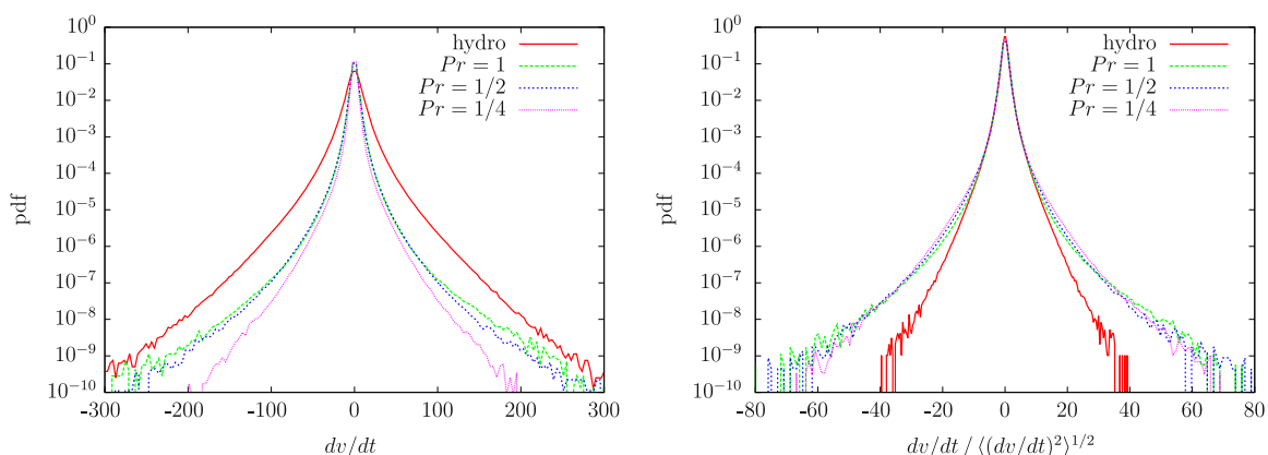
Figure 5. Probability distribution function of acceleration. Non-normalized (left) and normalized to standard deviation (right) for a hydrodynamic simulation (run tgH) and saturated regimes (run tg1, tg2 and tg3).
