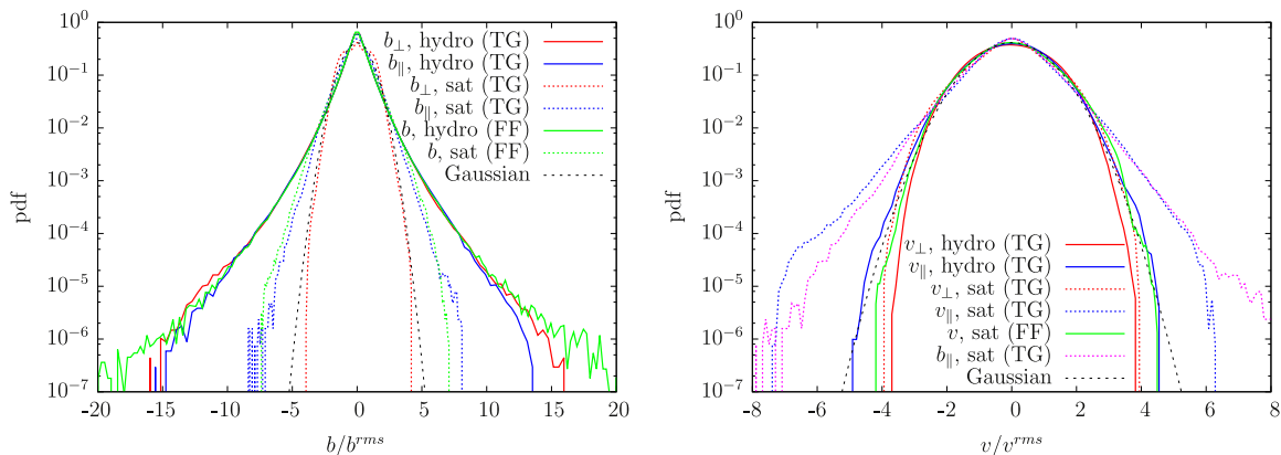
Figure 3. Probability distribution function of the magnetic field (left) and the velocity field (right) where the magnetic field component b_{\parallel, \text{sat}} (TG) is added for comparison. The data of the saturated Taylor–Green regime is from run tg3.
